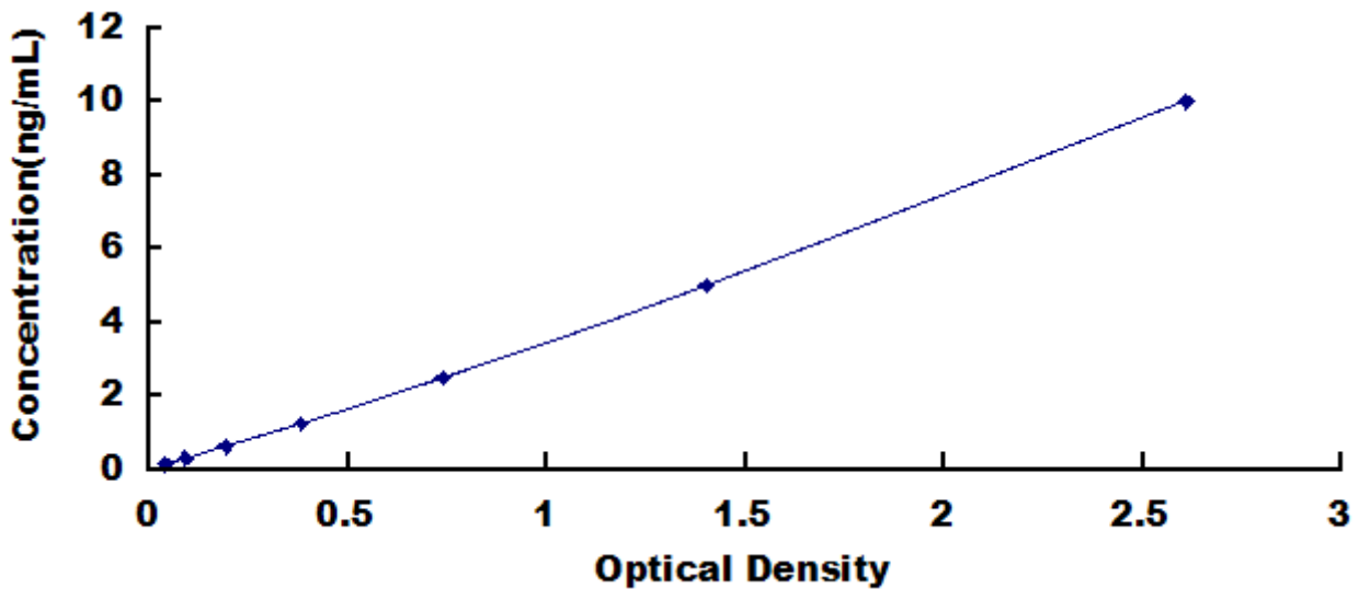
Typical Standard Curve for PRH2, Human ELISA.
