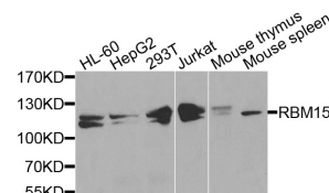
Western blot - RBM15 Polyclonal Antibody (A4936)
