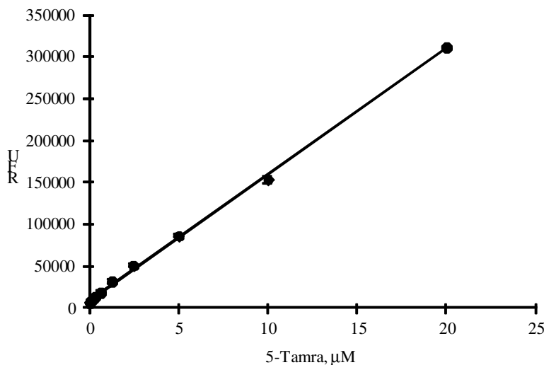
Figure 2. 5-TAMRA standard. 5-TAMRA was serially diluted in assay buffer containing substrate (FlexStation 384II, Molecular Devices; Ex/Em=540nm/575 nm, cut off 570nm)
