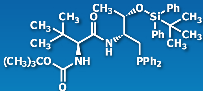
O-TBDPS-D-Thr-N-Boc-L-tert-Leu-Diphenylphosphine
