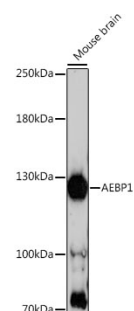
Western blot - AEBP1 Polyclonal Antibody (A16340)
