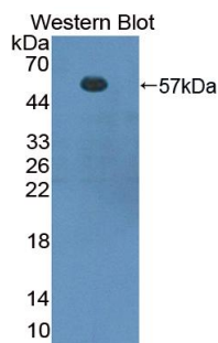
Figure. Western Blot; Sample: Recombinant FOXP3, Mouse.
