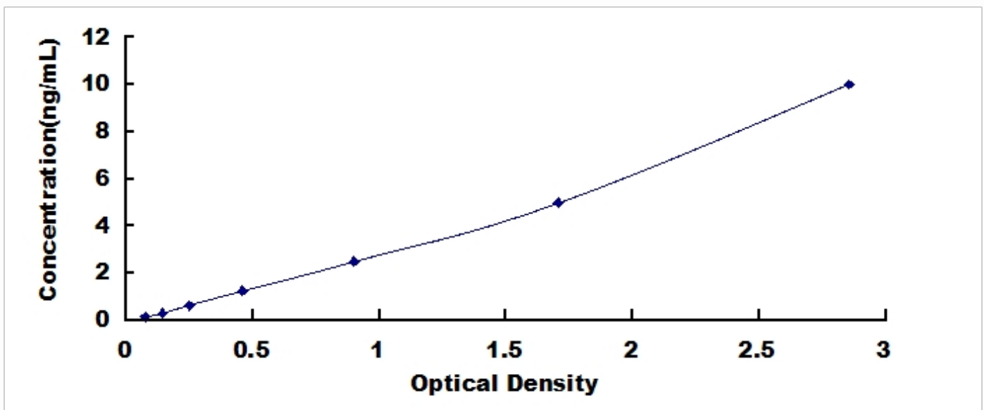
Typical Standard Curve for Transferrin, Mouse ELISA.
