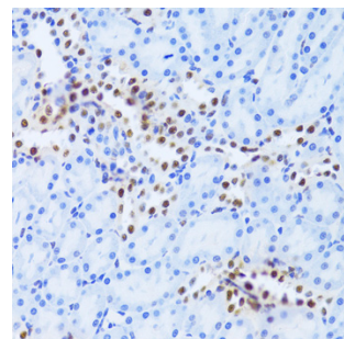
Immunohistochemistry - ANP32A Polyclonal Antibody (A5768)
