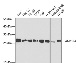
Western blot - ANP32A Polyclonal Antibody (A5768)
