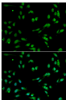
Immunofluorescence - ANP32A Polyclonal Antibody (A5768)
