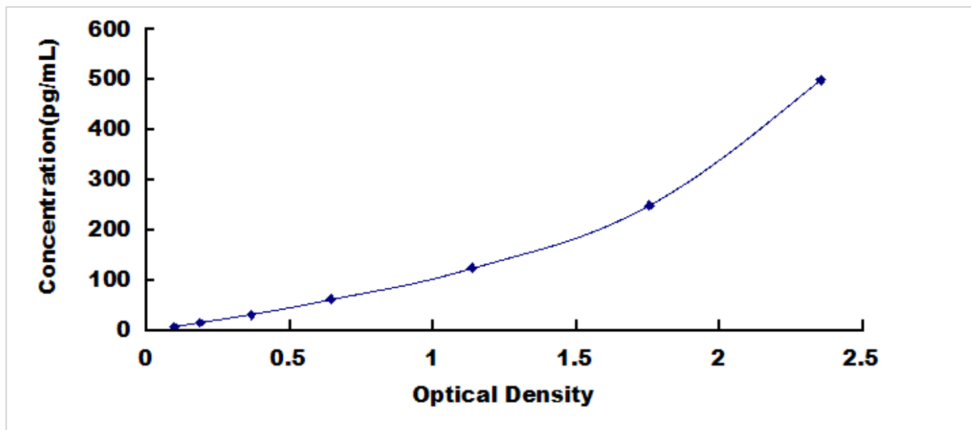
Typical Standard Curve for IL23, Human ELISA.
