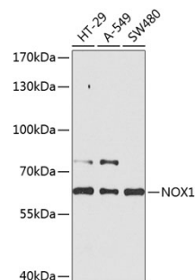
Western blot - NOX1 Polyclonal Antibody (A8527)
