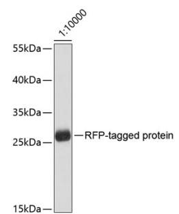
Western blot - Mouse anti RFP-Tag mAb (AE020)
