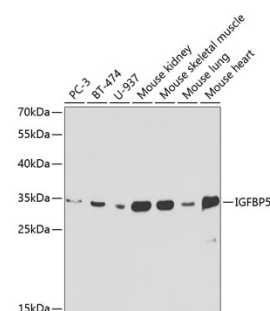
Western blot - IGFBP5 Polyclonal Antibody (A1720)
